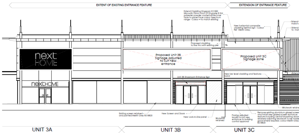
FRONT ELEVATION 1:100
